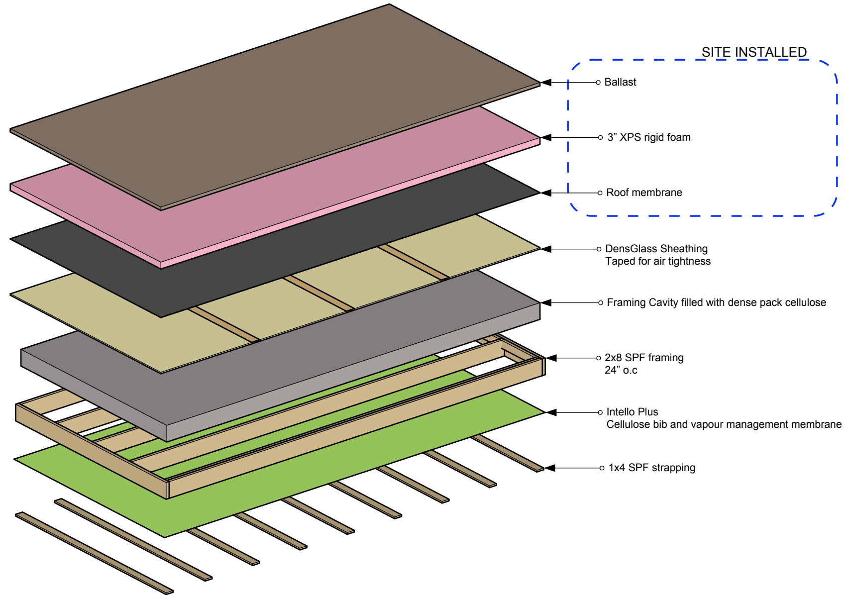
Exploded View
